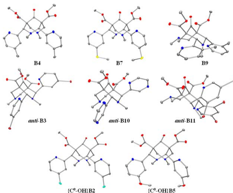
Figure 2. Experimental structures of the bispidones: syn -bispidones B4, B7, and B9; anti -bispidones B3, B10, and B11; C 9 -reduced syn -bispidones {C 9 -OH}B2 and {C 9 -OH}B5. Ellipsoids are shown at the 30% probability level; cocrystallized solvent molecules and hydrogen atoms are omitted for clarity.
