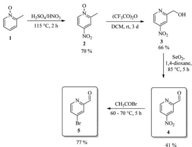
Scheme 1. Synthesis of 4-Nitro and 4-Prompicolinaldehyde (4 and 5, Respectively)
